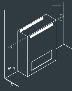
Minimum enclosure with front and back vents
